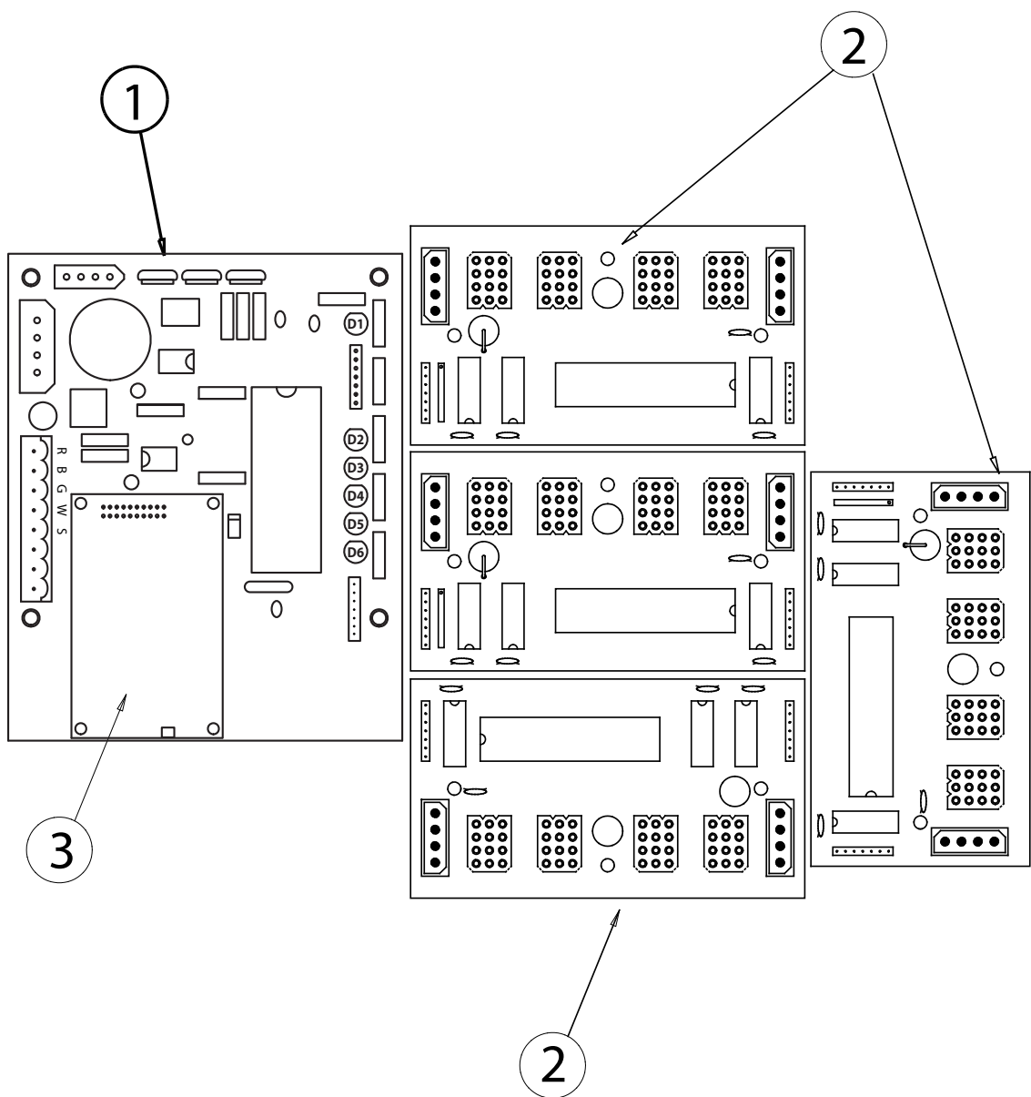
figure 2 CONTROLLER ASSEMBLY
