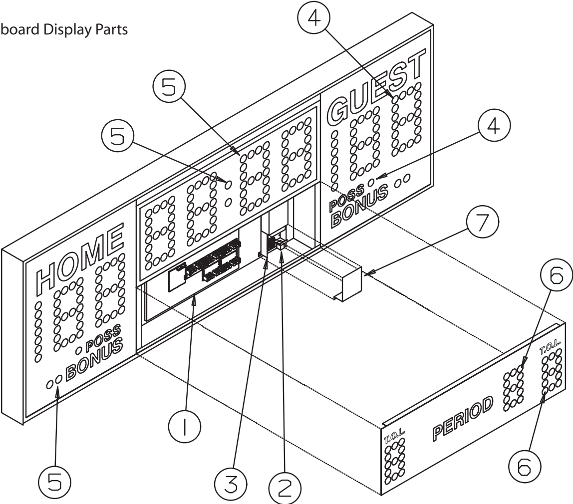
Figure 1 DISPLAY ASSEMBLY
